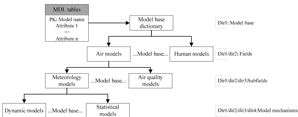
Figure 2. Model organization in model base.
